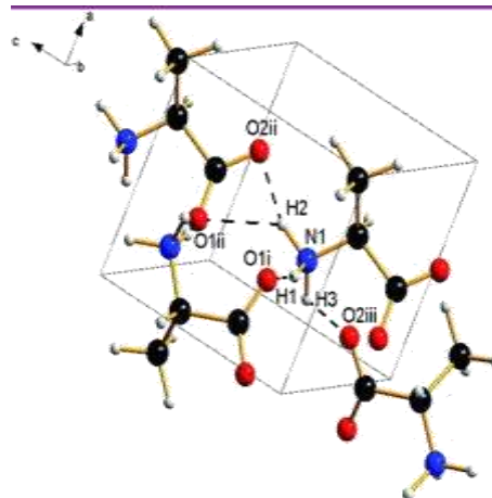
Figure 3: structure of crystal.
