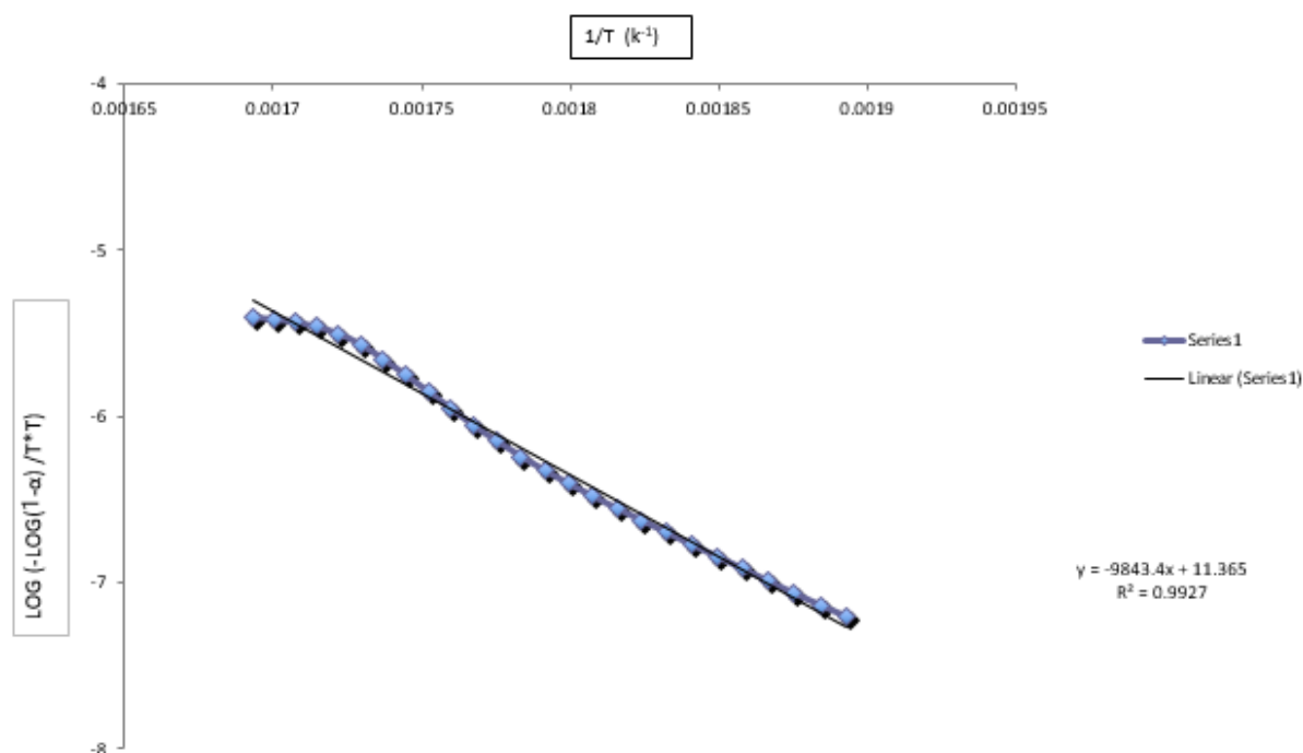
Figure 9: Graph \text{LOG}(-\text{LOG}(1-a)/T^*T) vs 1/T
