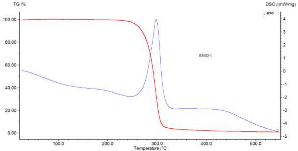
Figure 7 :Thermogram of Mg doped LAHC Crystal
